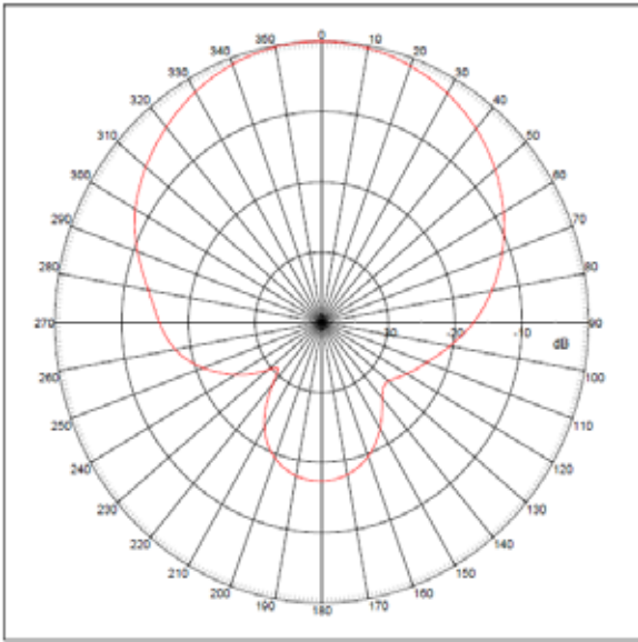
Linear A Peak Gain Angle = 359 deg Beam Width = 70.05 deg
