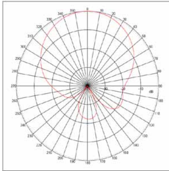
Linear B Peak Gain Angle = 0 deg Beam Width = 63.83 deg
